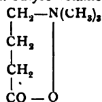
\gamma -n-butyro-betaine.
